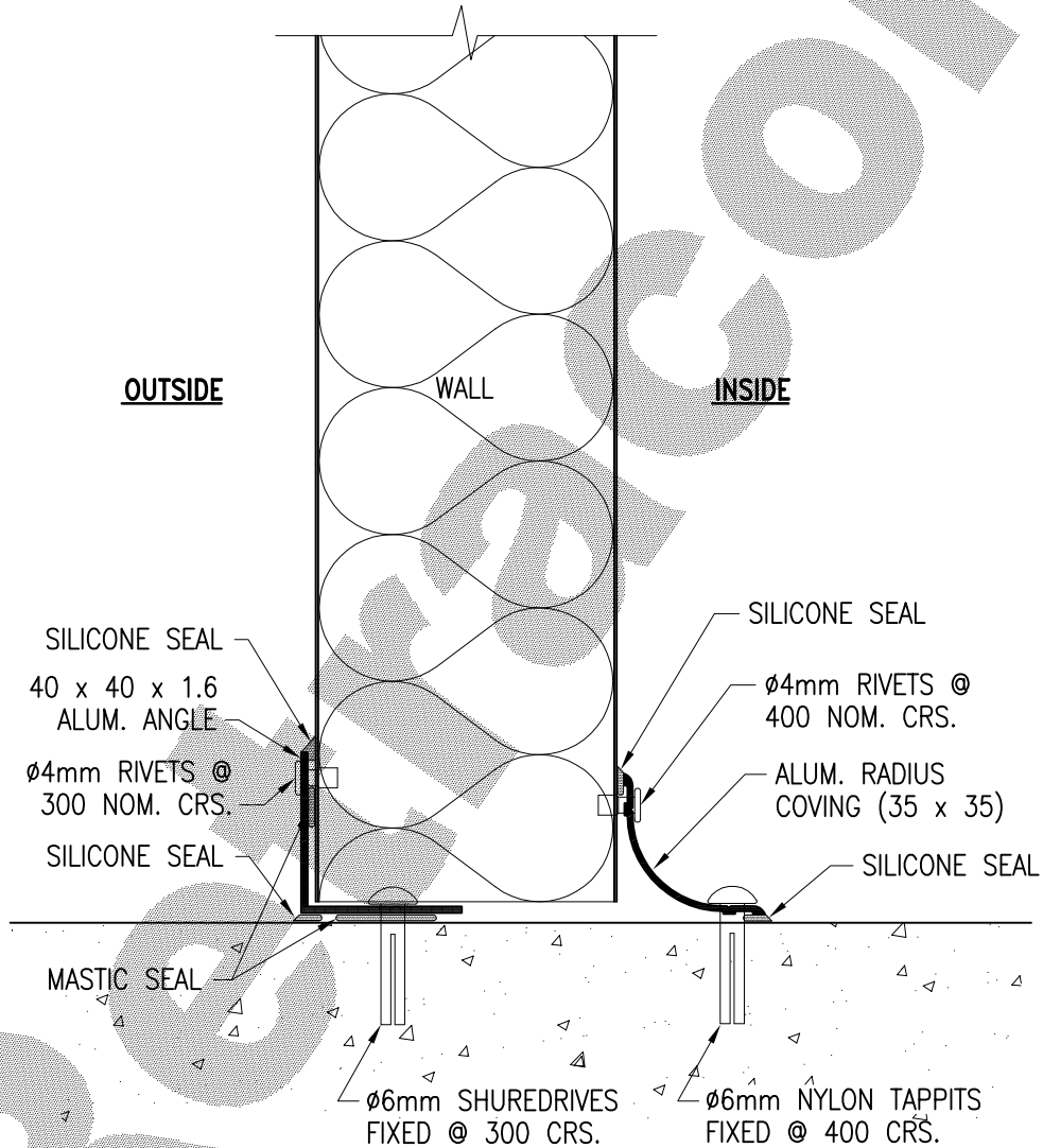
SECTIONAL VIEW
