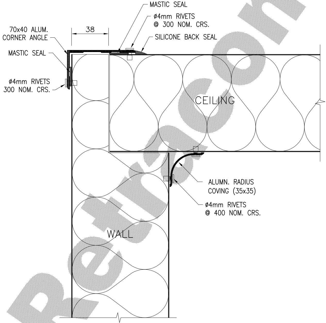
SECTIONAL VIEW
